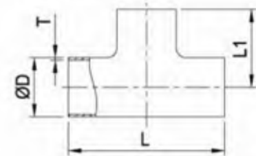
AS ET 短三通
