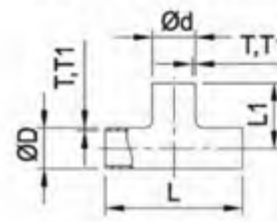
SMS PT 等径平口三通 SMS PT Tee Without Straight-End
