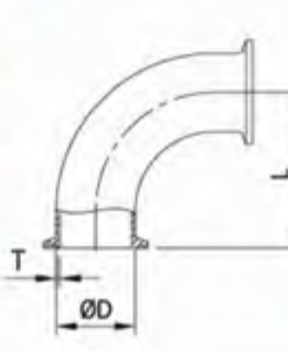
90° Clamp Bend
