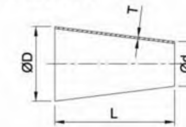
AS CR 同心大小头 Concentric Reducer
