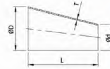
Eccentric Reducer
