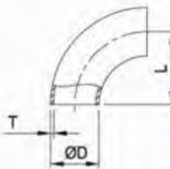
90° short bend
