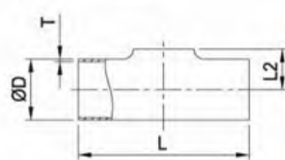
AS PT 平口三通
