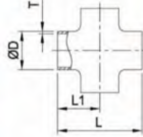
Short Cross AS ECS
