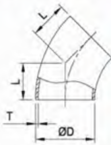
45° short elbow
