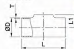
Pull Tee
