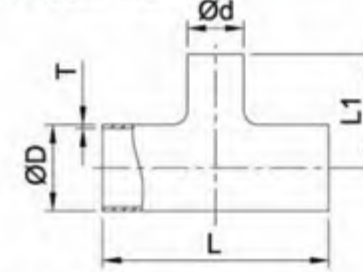
AS RTP 变径平口三通
