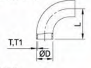
90长弯头 SMS 90 LB 90° Long Elbow
