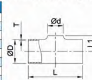
Reducing Tee W/O Straight End
