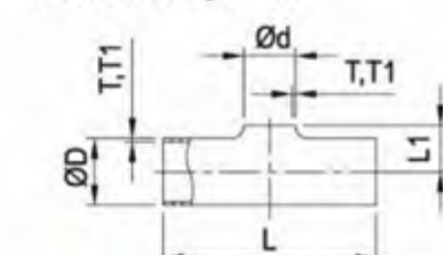
SMS PRT 变径平口三通 SMS PRT Welding Reducing Tee Without Straight-End
