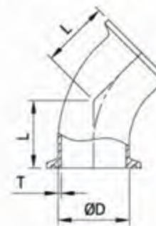
45° Clamp Elbow
