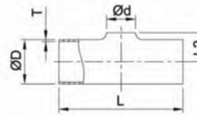
AS RTP 变径平口三通
