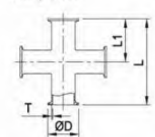
夹式长四通 C.9MP-Clamp Long Cross
